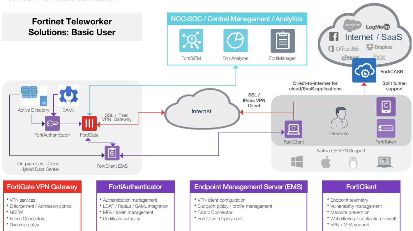
Figure 1: Notional Fortinet solution deployment for basic teleworker.
