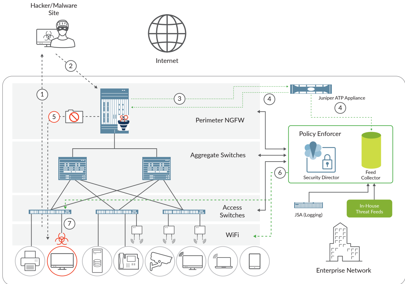
Figure 4: Secure Network Deployment with Juniper Connected Security and Juniper ATP Appliance
