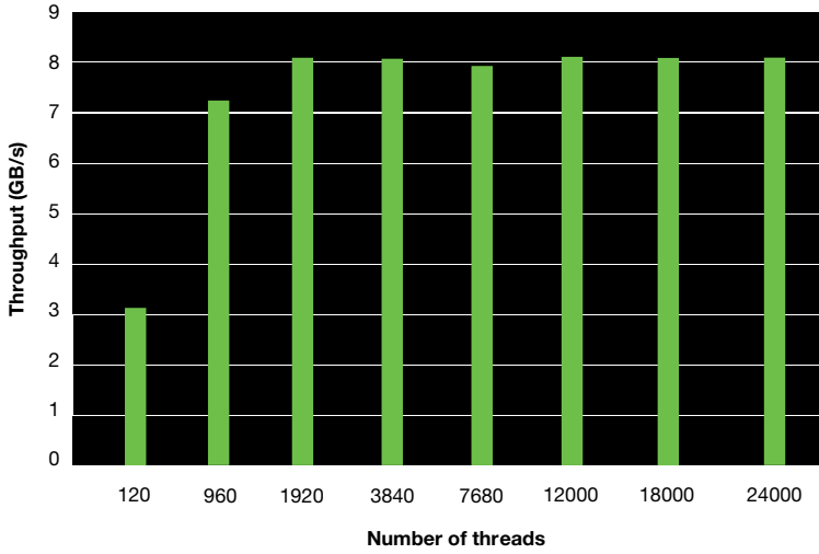
4+2 erasure code read performance, 8MB object size
